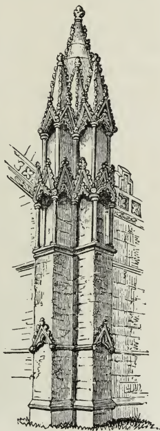
147. Gadsby, Leicestershire, c. 1350. Corner buttress with canopies and pinnacle.
